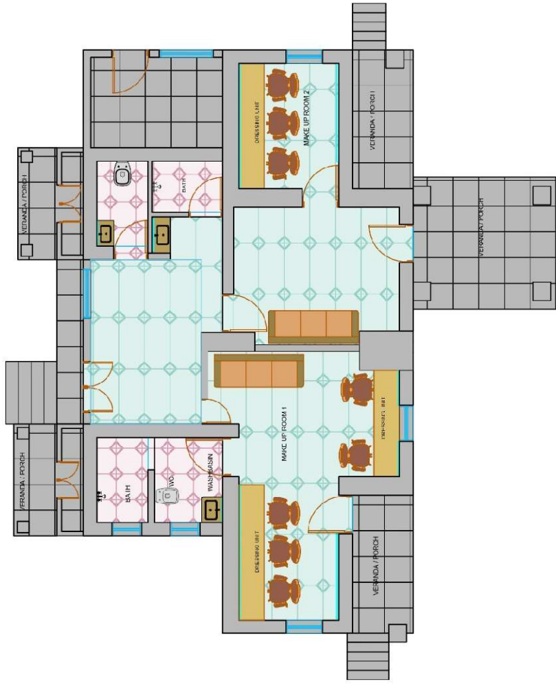
P31 FLOOR PLAN
